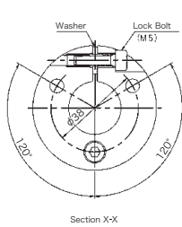
Section X-X
